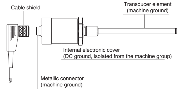
Connector output SK4-A-A/B/C/H
