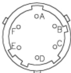
6-poliger Steckverbinder PT06A-10-6S
