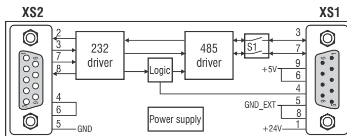
Schema a blocchi / Block diagram
